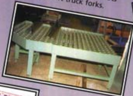
Special die table with slots for fork-lift truck forks.
